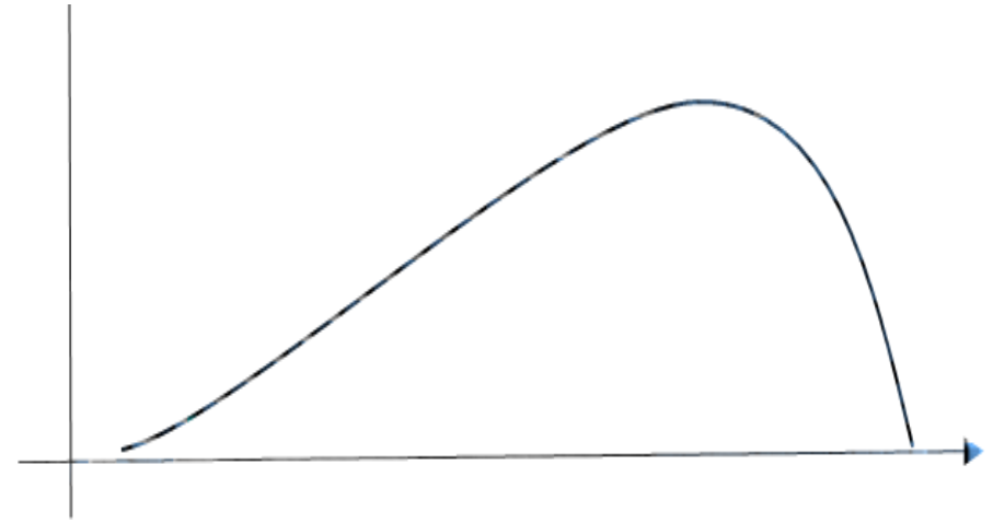
Left(Negative) Skewness
