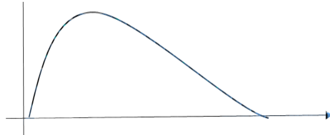
Right(Positive) Skewness
