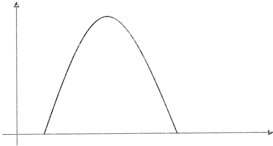
Normally distributed (Gaussian Curve)
